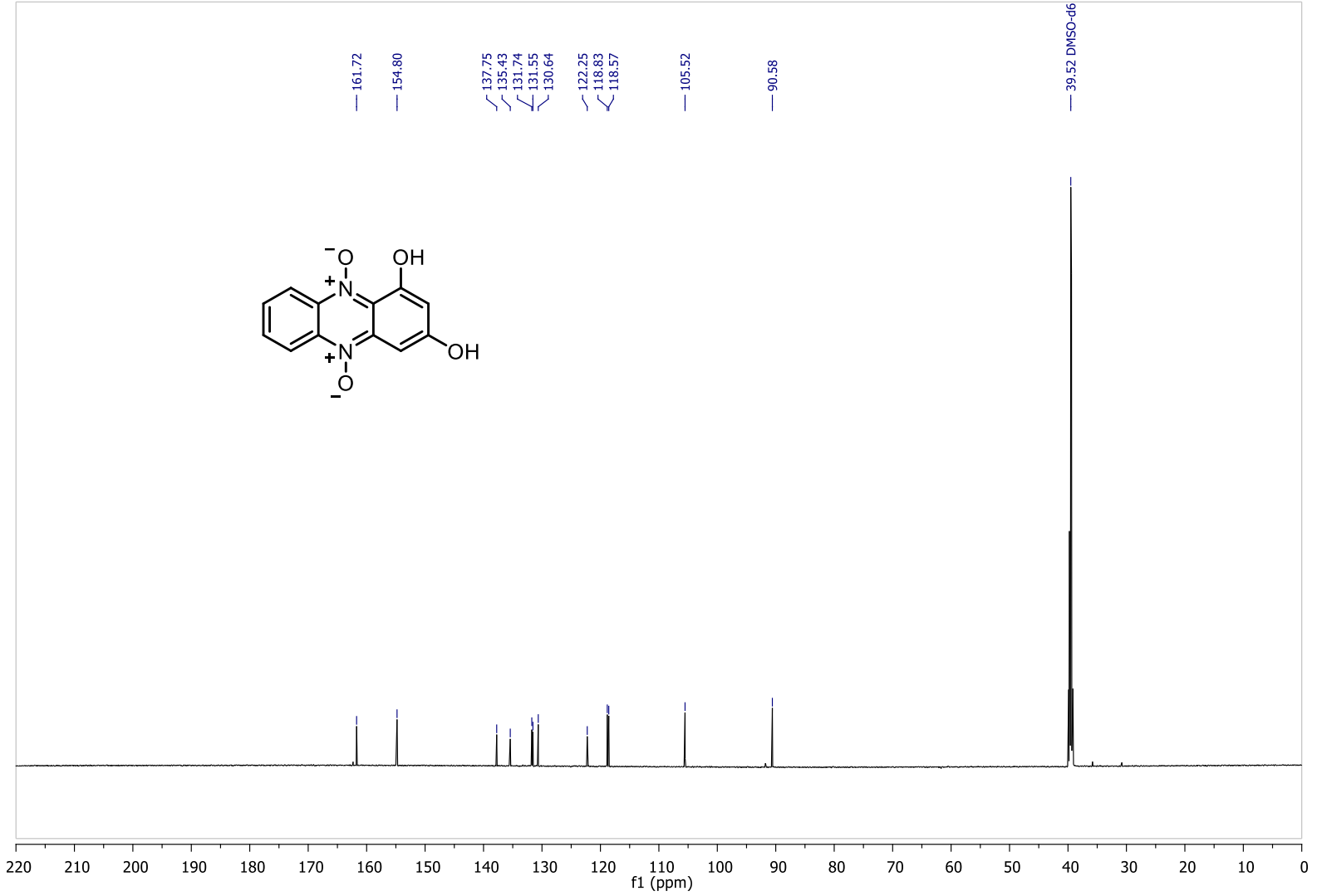
^{13}\text{C} NMR of 1,3-dihydroxyphenazine dioxide in \text{d}_6\text{-DMSO} following recrystallization from DMF/water.
